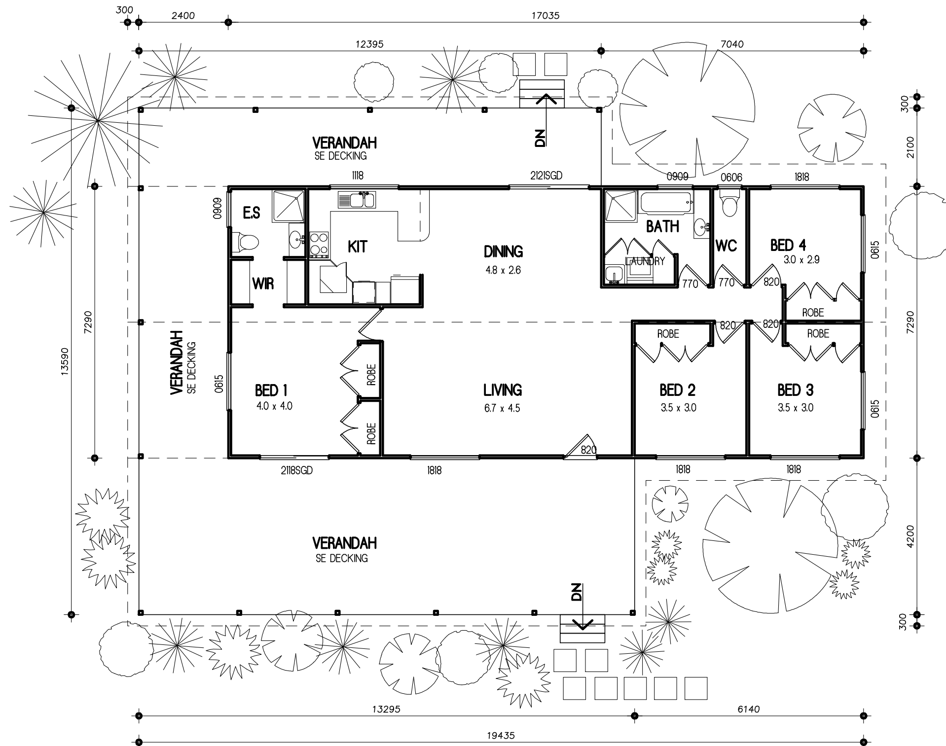
FLOOR PLAN SCALE 1:100
