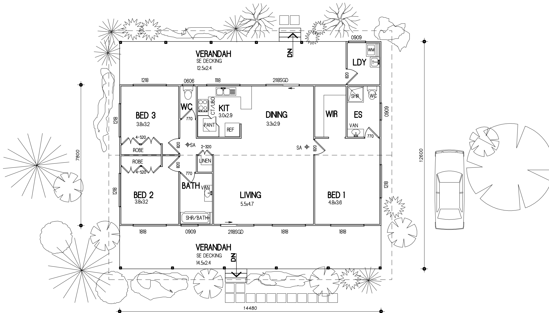
FLOOR PLAN SCALE 1:100
