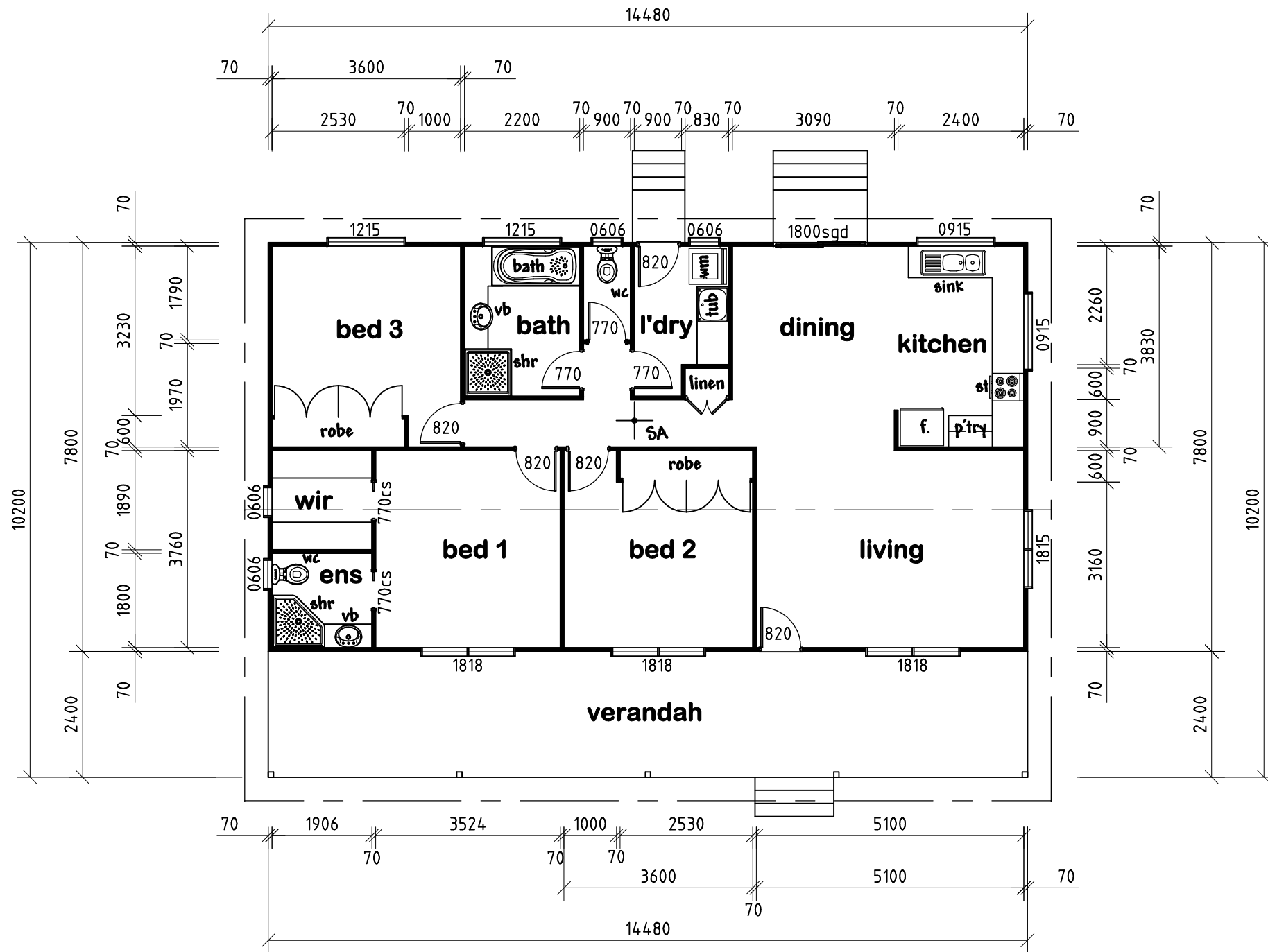
floor plan
